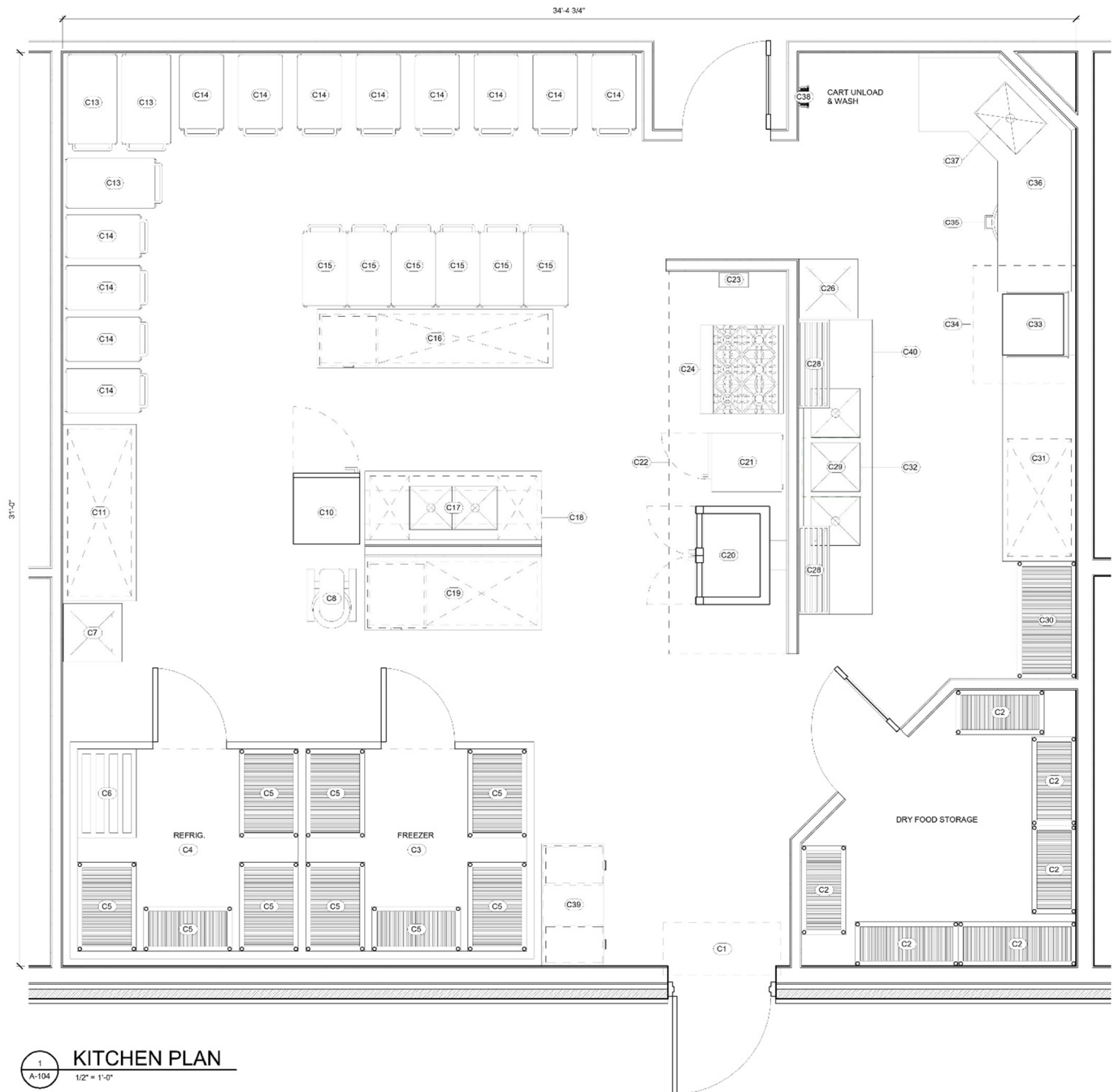
Kitchen – Large 338 Child Facility
